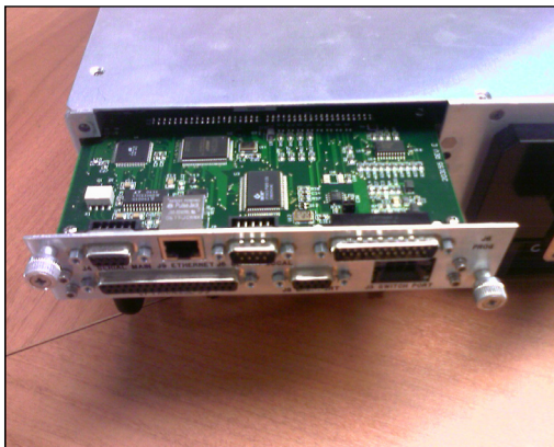
Removable rear panel monitor and control card
